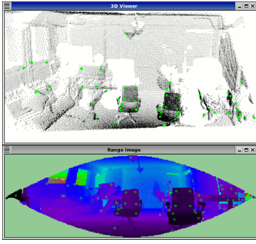
Fig. 3. A point cloud made from a single 3D image. The blank parts of the point cloud is where the sight was blocked by objects. Source: http://www.cs.technion.ac.il/cs236329/tutorials/ICP.pdf
