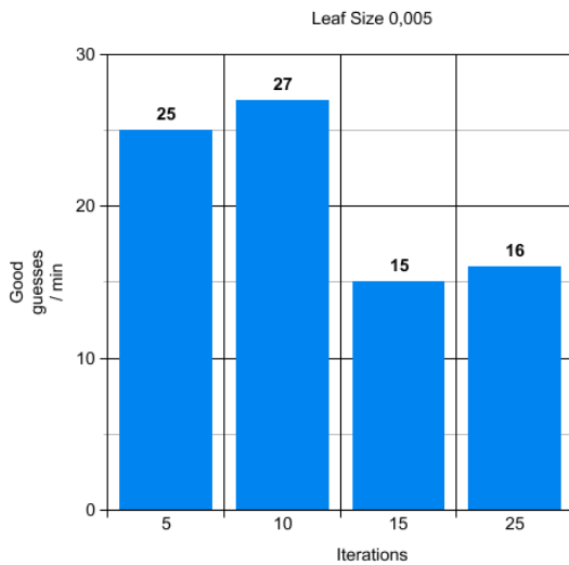
Fig. 11. Graph showing results with leaf size 0,005. Good guesses per minute is shown based on number of iterations.
