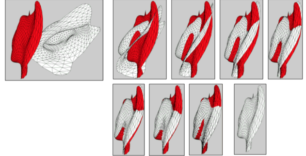
Fig. 5. A rotated hat is gradually fitted to its template, giving the placement of the hat compared to the initial placement. Source: http://www.cs.technion.ac.il/cs236329/tutorials/ICP.pdf
