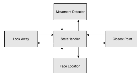
Figure 4: This is a complement to Figure 3. These dependencies are not shown in Fig. 3 to allow for more clarity. Nevertheless, these dependencies do still exist.
