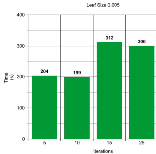
Fig. 13. Graph showing compute time with leaf size 0,005. Compute time is shown based on number of iterations.
